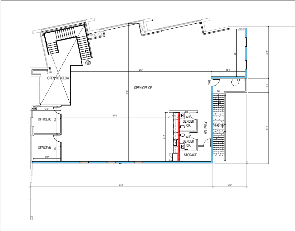
MEZZANINE OFFICE PLAN ±4,504 SF
